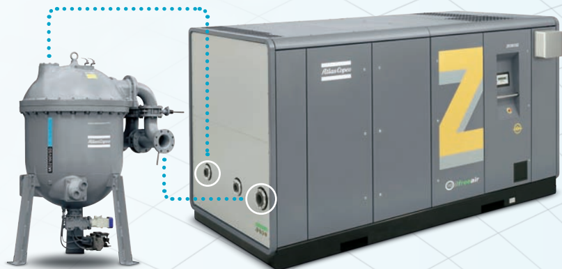
ZR 700 VSD with external MD 2100 VSD dryer
